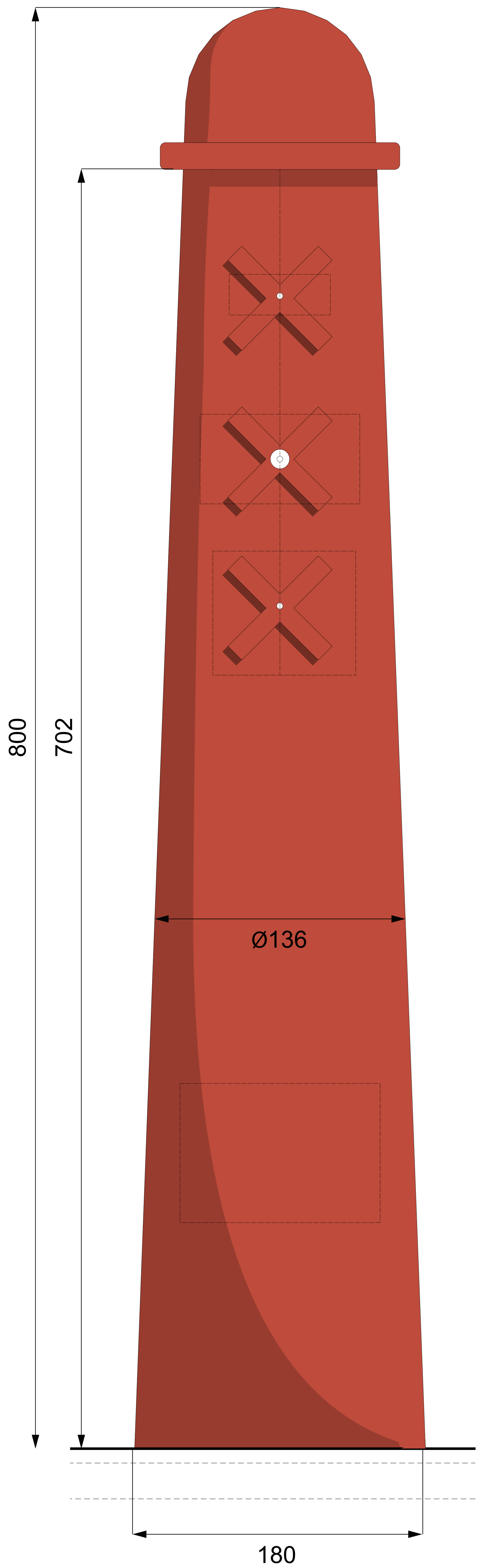
FRONT ELEVATION & SECTION DETAIL 1:1 at A0
